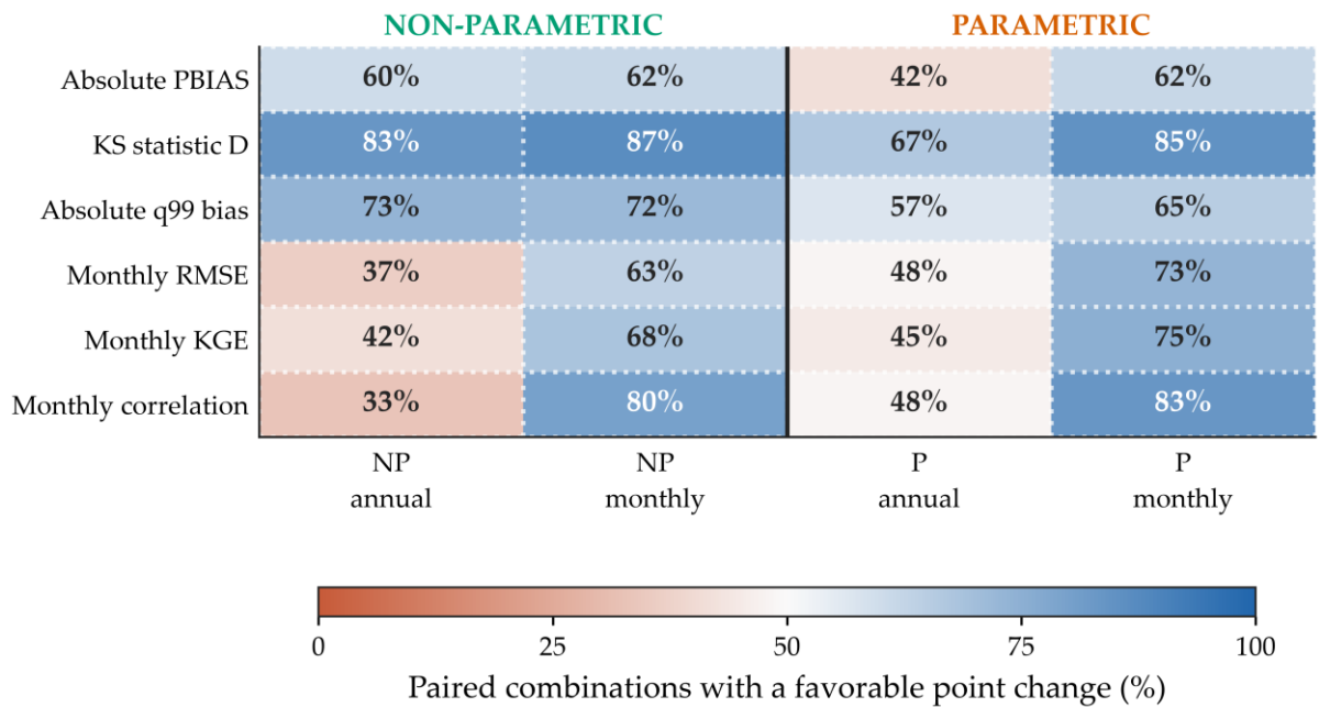
Figure 5. Percentage of 60 paired model-station evaluations with a favorable point change relative to raw CMIP6 simulations. Values above 50% indicate a favorable change for most pairs; percentages are descriptive and pairs are not independent spatial replicates.
