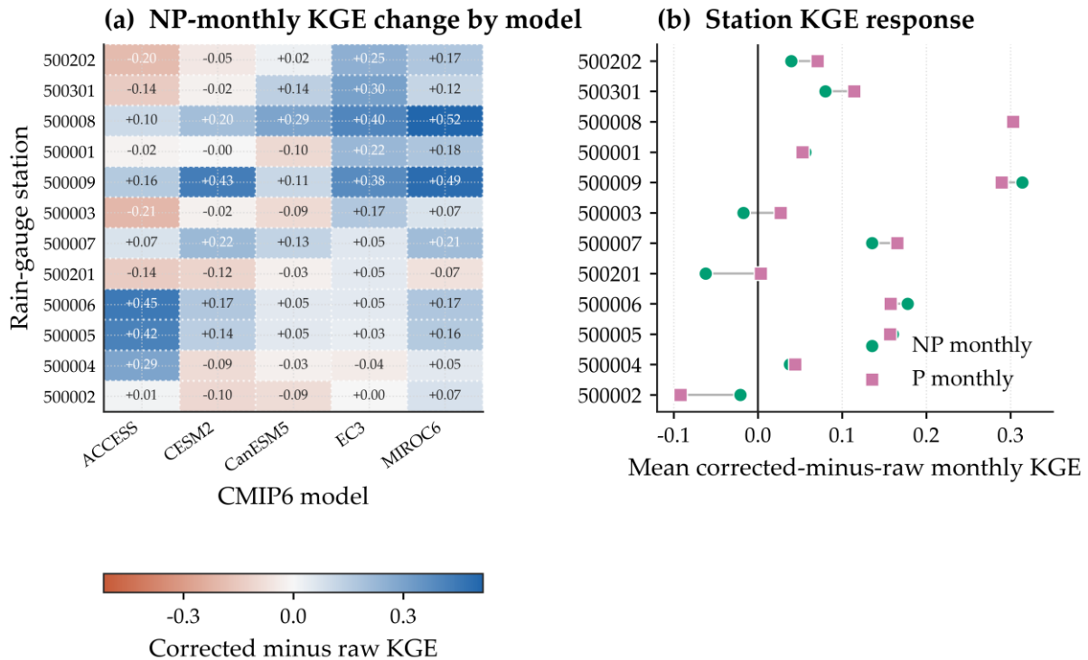
Figure 6. Station-level response of monthly QDM. (a) Heatmap of corrected-minus-row KGE for NP monthly QDM by station and CMIP6 model. (b) Paired station means for non-parametric and parametric monthly QDM. Values are descriptive because gauges share model grid cells; station patterns are not interpreted as causal geographic effects.
