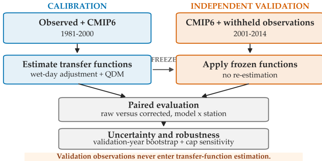
Figure 2. Fit-freeze-apply framework. Observation-dependent transfer functions were estimated in 1981-2000 and applied without re-estimation in 2001-2014; uncertainty used paired year-block bootstrap resampling.
